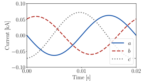
Fig. 6: A 3-phase capacitor with stationary unbalanced sinusoidal AC voltage is subject to the sum of a relative and a centrifugal current: \mathbf{i} = C\beta_\varphi \mathbf{v}_\parallel + C\boldsymbol{\omega}_\varphi \times (\boldsymbol{\omega}_\varphi \times \boldsymbol{\varphi}) . The Coriolis and Euler components cancel out each other.
